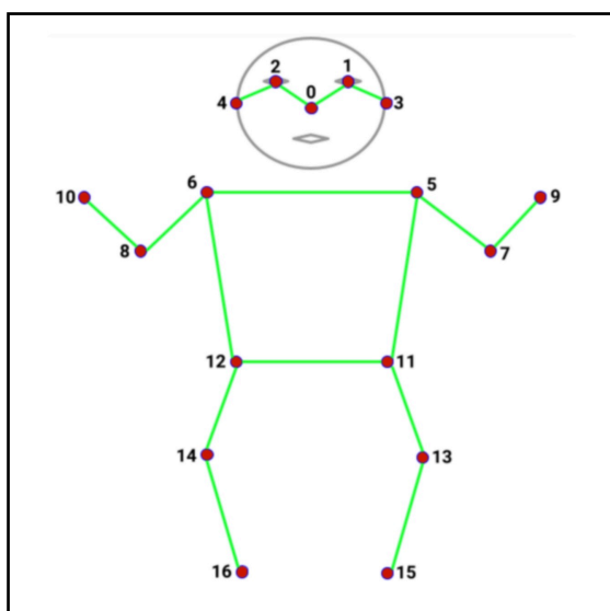
Figure 1 BodyPose('moveNet')
