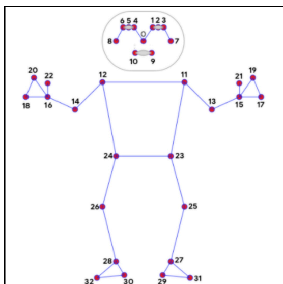
Figure 2 BodyPose('blazePose')
