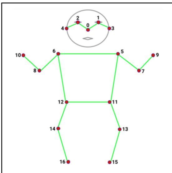
Figure 1 BodyPose('moveNet')
