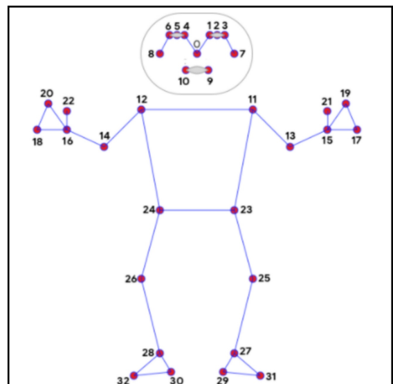
Figure 2 BodyPose('blazePose')
