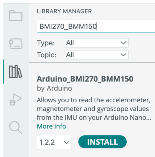
Figure 1: library manager
