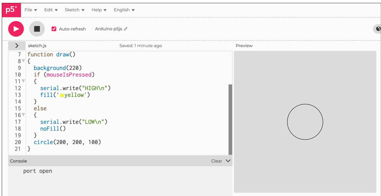
Figure B1.13b: mouse not pressed
