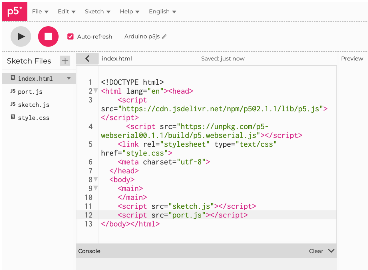
Figure 2: webserial and port.js to index.html
