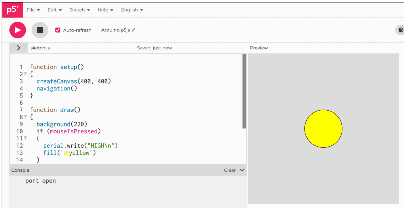
Figure B1.13a: mouse pressed
