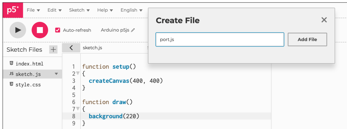
Figure 1: port.js file
