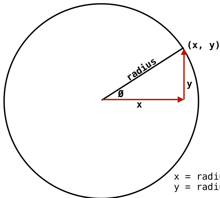
Figure 2: coordinates of a point on a circle
